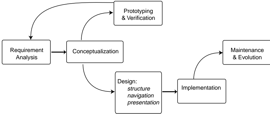
Figure 1. The lifecycle of a Web application.
